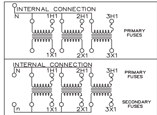
CONNECTION DIAGRAMS
