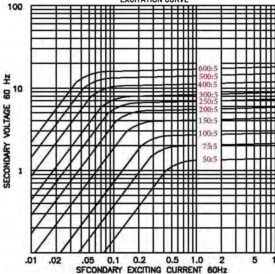
EXCITATION CURVE
