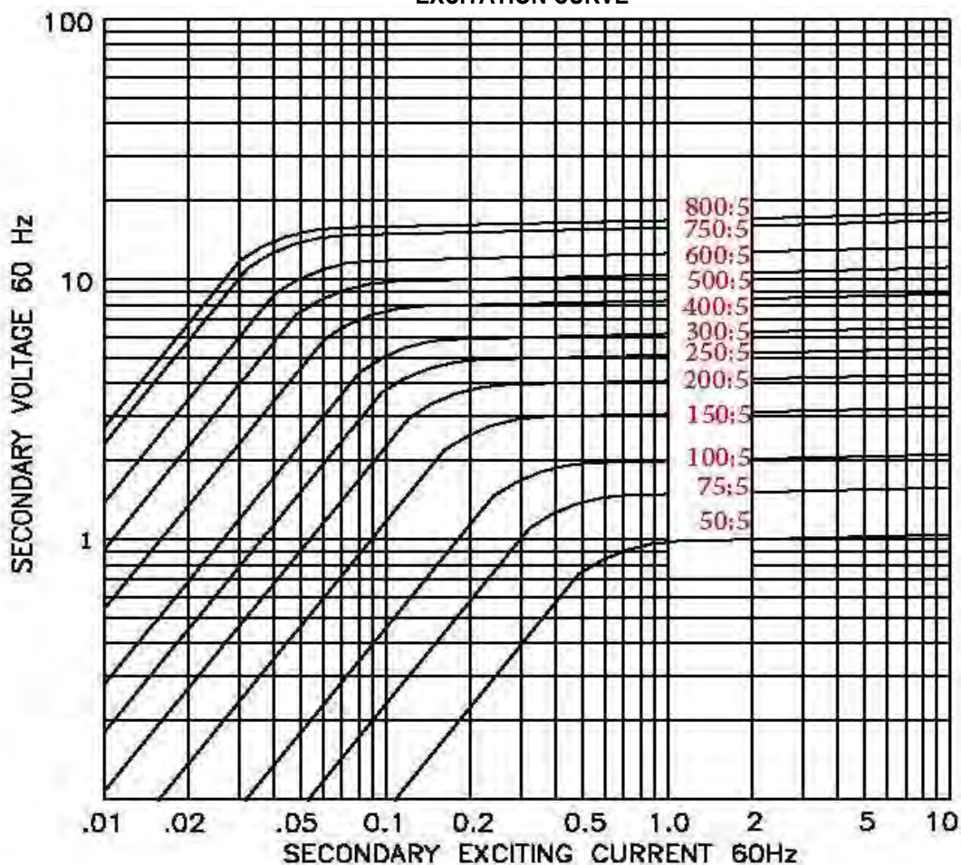
EXCITATION CURVE
