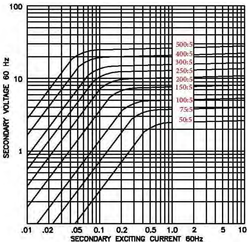
EXCITATION CURVE
